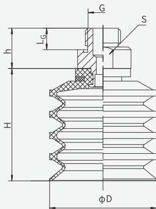
SBL30-50 Male connection
