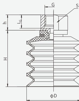
SBL30-50 Female connection
