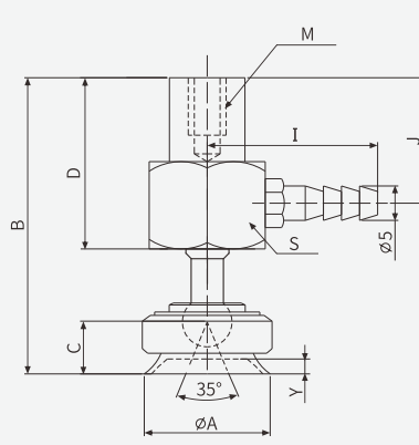
Suction cup diameter 20–50
