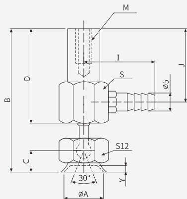
Suction cup diameter 10–15
