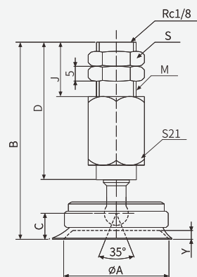
Suction cup diameter 60-100
