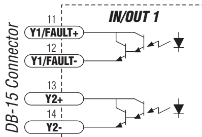
Sample Connection
