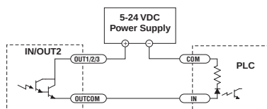
OUT1,OUT2,OUT3 Sourcing Output
