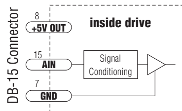
Connecting a Potentiometer
