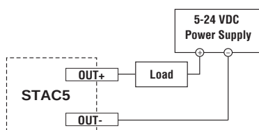
Y1, Y2, OUT4 Sinking Output
