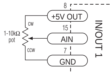
Connecting a Potentiometer
