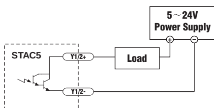
Sourcing Output
