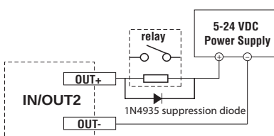
Driving a Relay Using Y1, Y2, or OUT4
