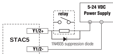
Driving a Relay
