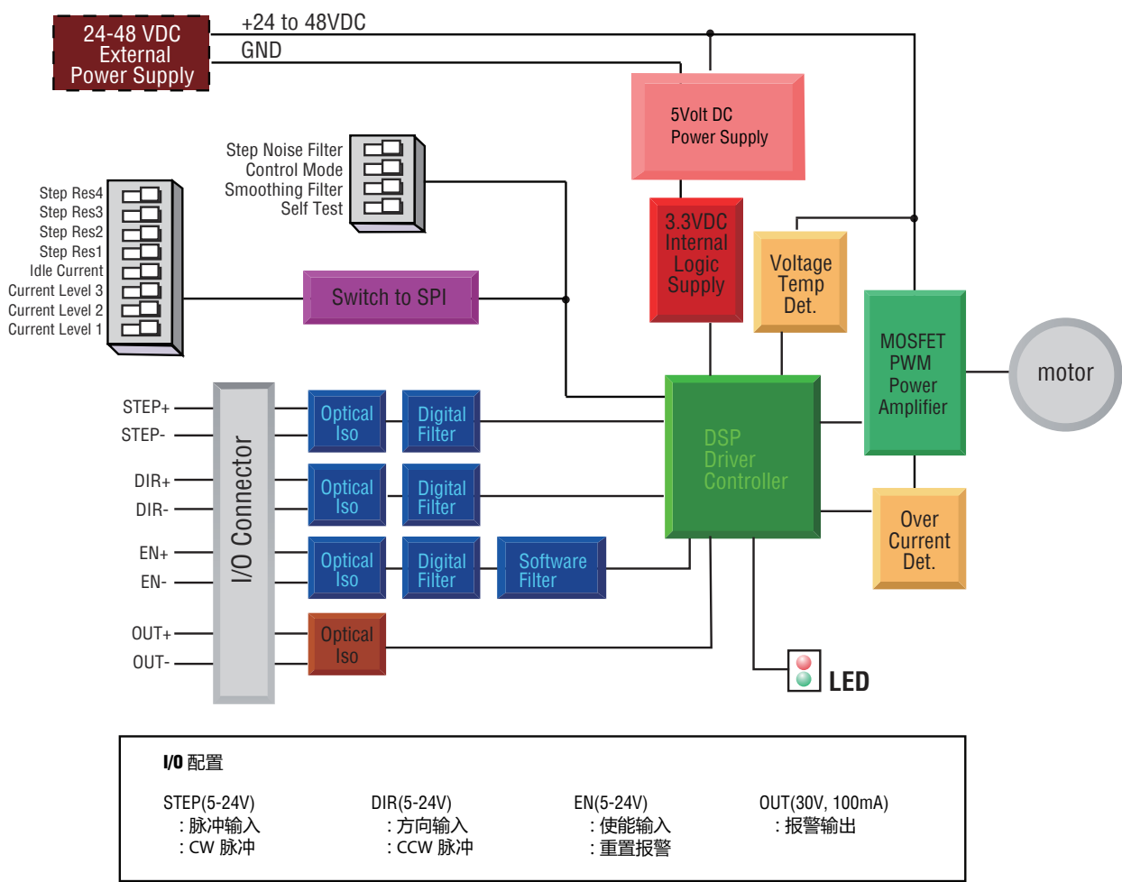
SRX04 Block Diagram
