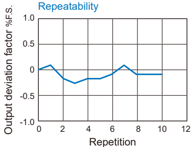
Repeatability
