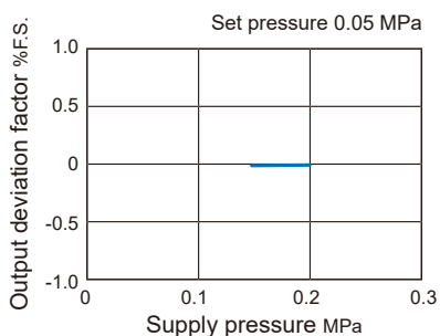
Pressure characteristics
