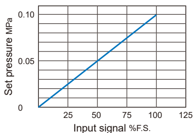
Linearity
