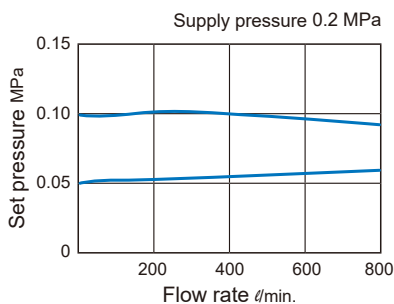
Flow rate characteristics
