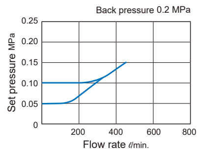
Relief flow characteristics
